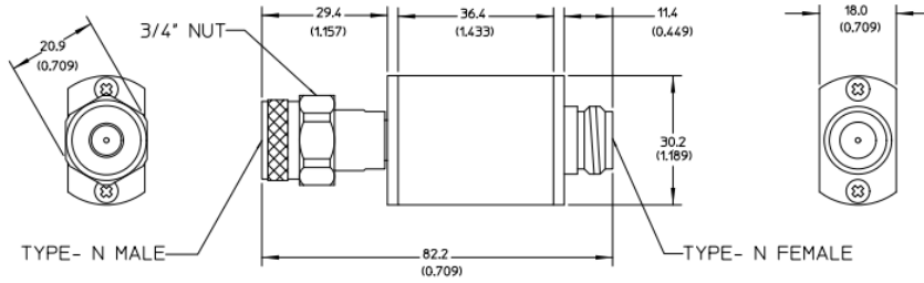
Figure 13. N9355/6B mechanical dimension
